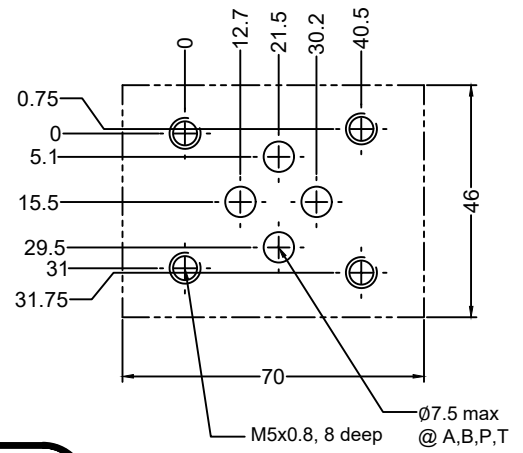
Subplate Mounting Interface TCM06**
