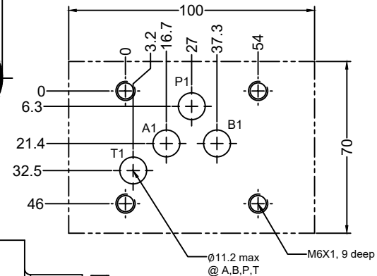
Subplate Mounting Interface TCM10**
